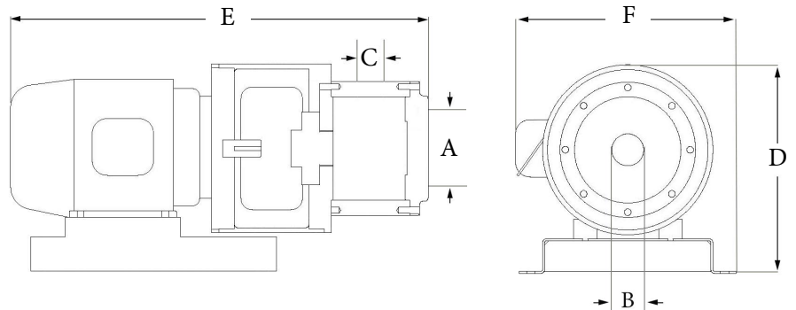
Series 400 Direct Driven (Models 401-430)
