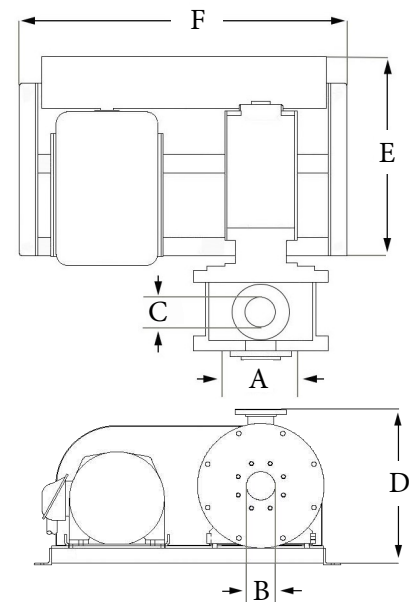
Series 400 Belt Driven (Models 450-4100)
